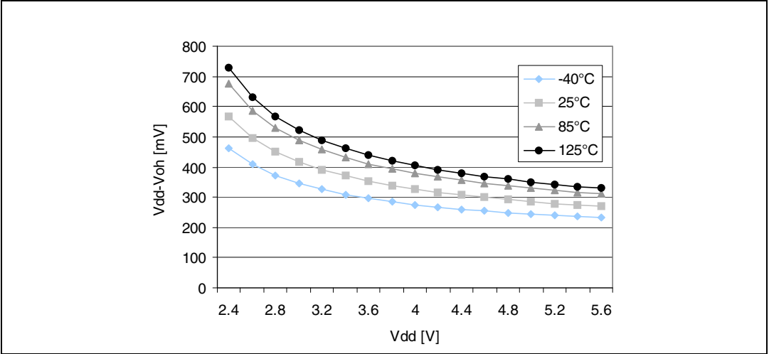
Figure 94. Typical V_{DD}-V_{OH} vs. V_{DD} at I_{IO} = 2\text{ mA} (high sink)
