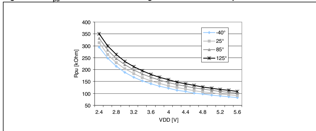
Figure 75. R_{pu} resistance versus voltage at four different temperatures
